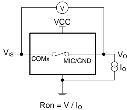
ON-Resistance ( R_{ON} )
